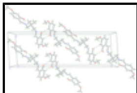
Fig. 2. The crystal packing of the title compound, viewed down the b -axis, showing the R_2^2(8) dimers. Hydrogen bonds are shown as dashed lines.
