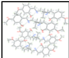
Fig. 1. The asymmetric unit of the title compound, showing four independent molecules with atom labels. Displacement ellipsoids are drawn at the 40% probability level. Intramolecular interactions are shown as dashed lines.
